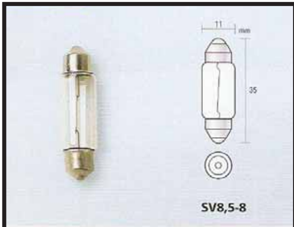
REF. 6458111 LAMPARA PLAFÓN 10W SV8,5 11X38MM
