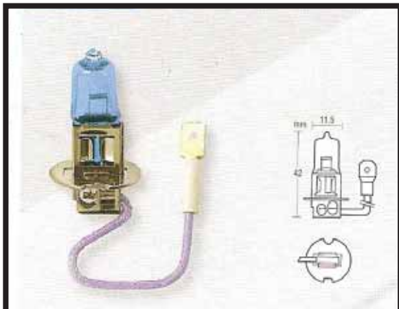
REF. 6458182 LAMPARA BLUE-XENON H3 12V 55W
