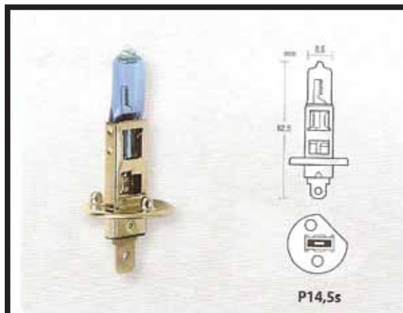
REF. 6458180 LAMPARA BLUE-XENON H1 12V 55W
