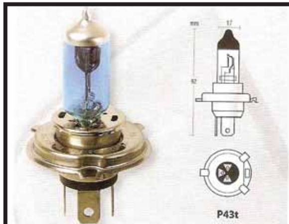
REF. 6458184 LAMPARA BLUE-XENON H4 12V 60-55W 2U
