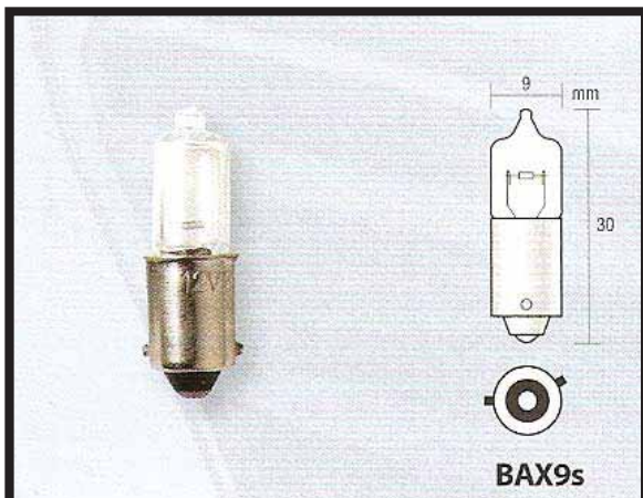
REF. 6458128 LAMPARA 12V H6W BLISTER 2P
